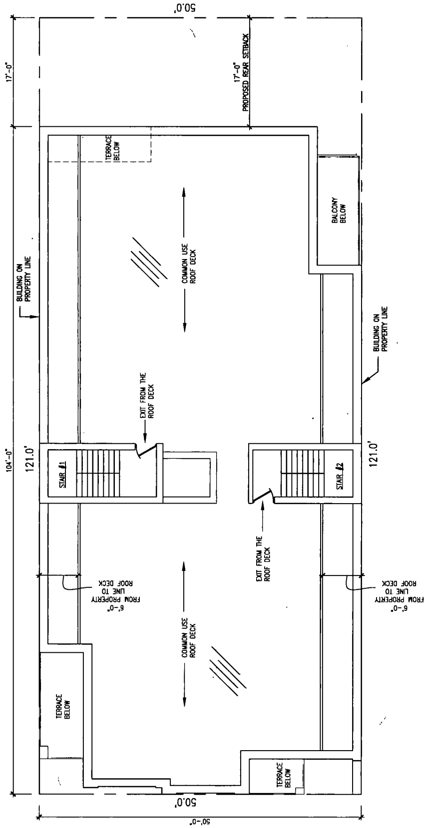
1 ROOF PLAN A1.3 SCALE: NONE
