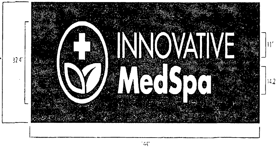
Flush mounted low voltage LED Channel Letters / Logo on 3" deep panel Aluminum returns/cans with acrylic faces and gemlite trim cap
