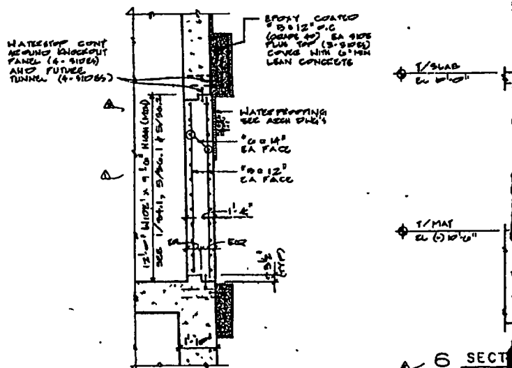
4 KNOCKOUT PANEL DETAIL
