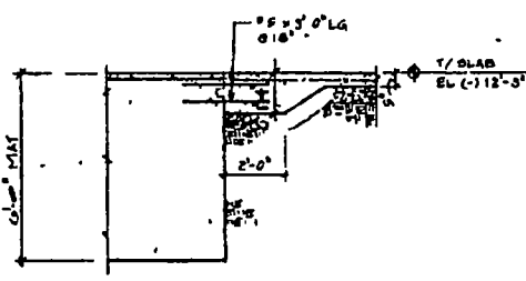
4 KNOCKOUT PANEL DETAIL
