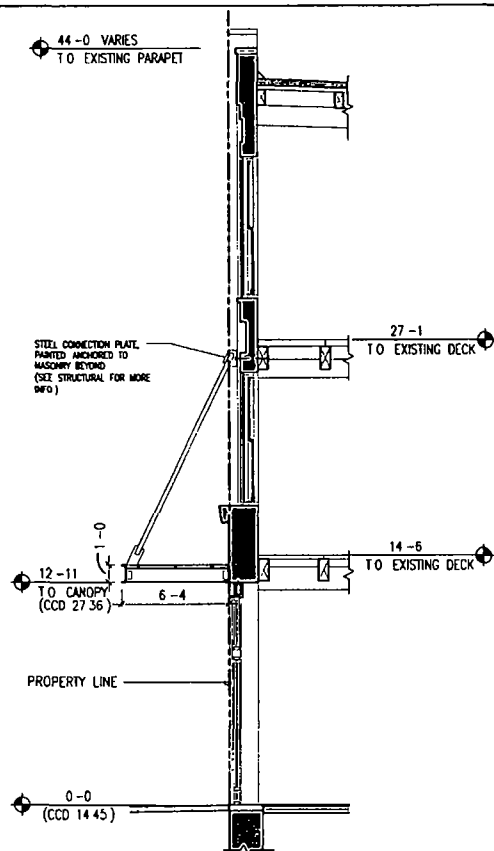
SECTION AT PROPOSED CANOPY SCALE 1/8" = 1'-0"
