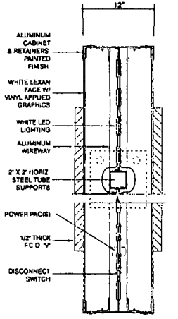
SIDE VIEW DETAIL NTS
