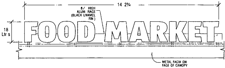
B LED Illum d Race Mount Letters on Canopy scale 1/2" = 1' 0" ONE(1) SET REQ'D WHITE PLEX FACES GRAY TRIM CAP & GRAY PTD ALUM CHANNEL (RETURNS) WHITE LED ILLUM
