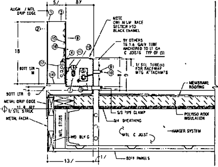
Letters w/ Race on Canopy SECTION CAULK PENETRATIONS scale 1" = 1' 0"
