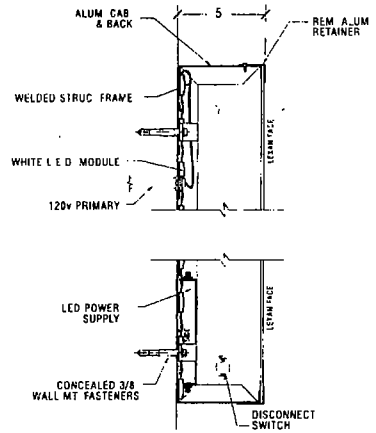
C Standard Lexan Face Illum d Wall Sign ONE(1) req'd scale 1/4" = 1' 0"
