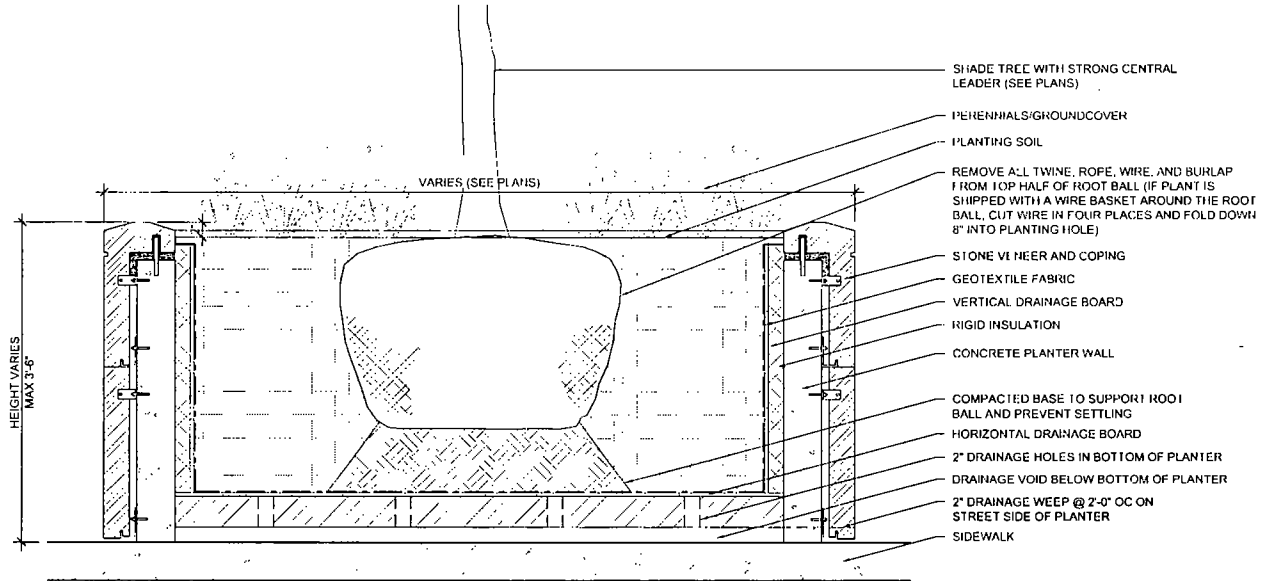
1 SIDEWALK PLANTER W/TREE SECTION 1/2" = 1'-0"
