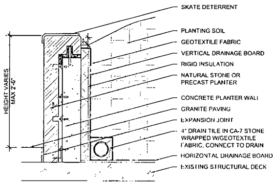
1 RAISED PLANTER SECTION 1/2" = 1'-0"
