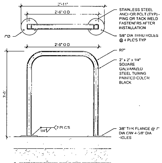
3 BIKE RACK DETAIL 1/2" = 1'-0"
