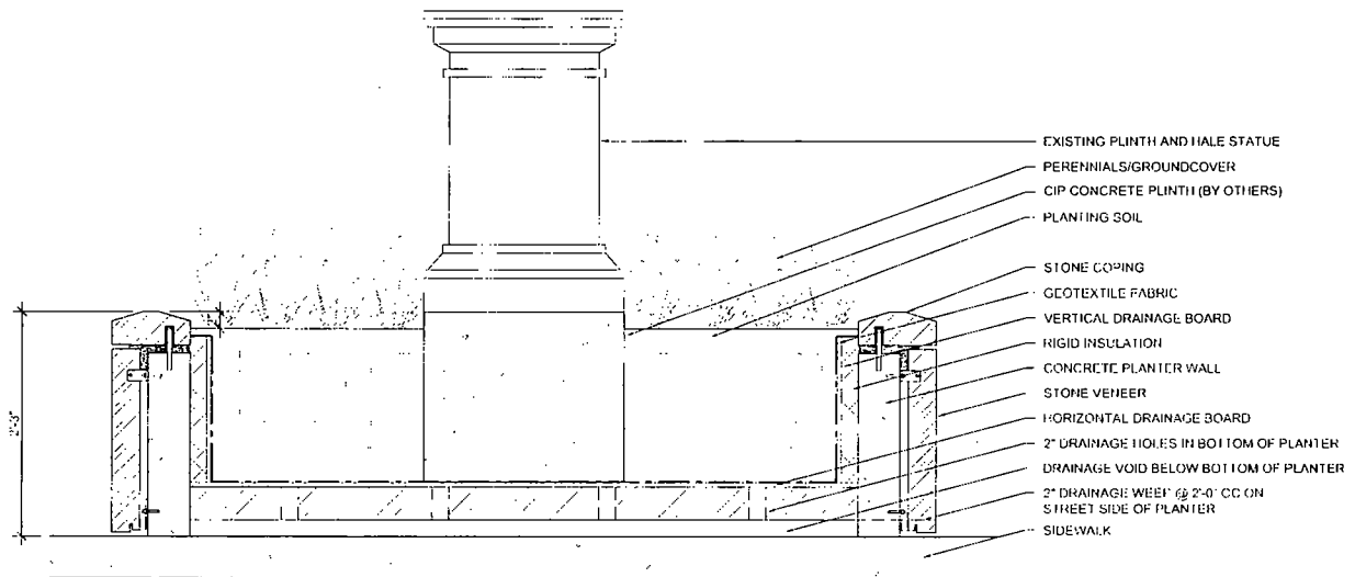
2 SIDEWALK PLANTER W/STATUE SECTION 1/2" = 1'-0"
