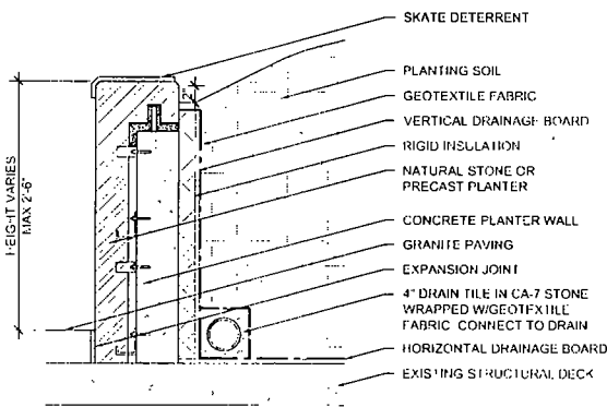
2 RAISED PLANTER SECTION 1/2" = 1'-0"
