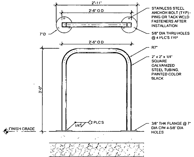
2 BIKE RACK DETAIL 1/2" = 1'-0"
