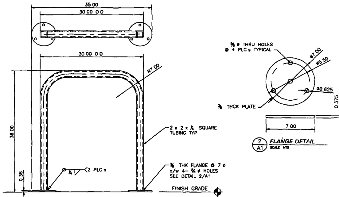
1 TYPE B BICYCLE RACK A1 SCALE 1 = 1 - 0
