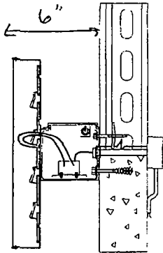
END VIEW SKELETON
