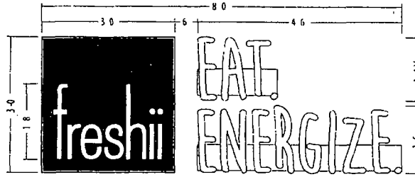
FRONT VIEW SCALE 3/4" = 1'-0" 240 SQ FT
