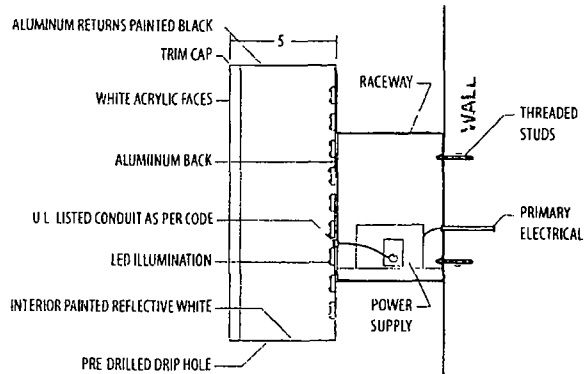
SIDE VIEW CHANNEL LETTERS SCALE 1/2" = 1'-0"
