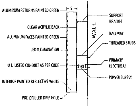
SIDE VIEW FRESHII LOGO SCALE 1" = 1'-0"
