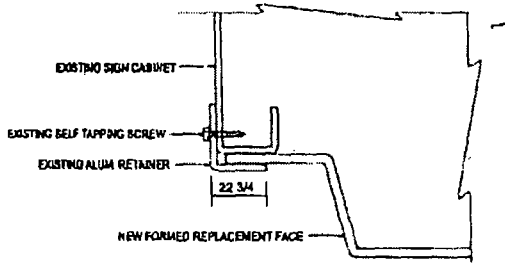
REPLACEMENT FACE ATTACHMENT DETAIL
