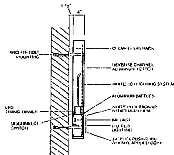
SECTION THRU CHANNEL LETTERS 3/4"
