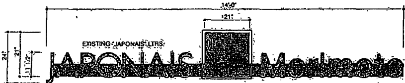
INDIVIDUAL INT. NEON ILLUMINATED LETTER & LOGO DISPLAY. 1/2" = 1'-0"
