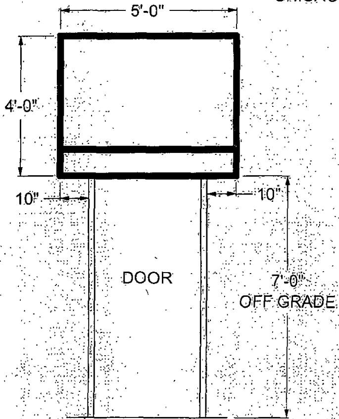
FRONT VIEW NORTH ELEVATION
