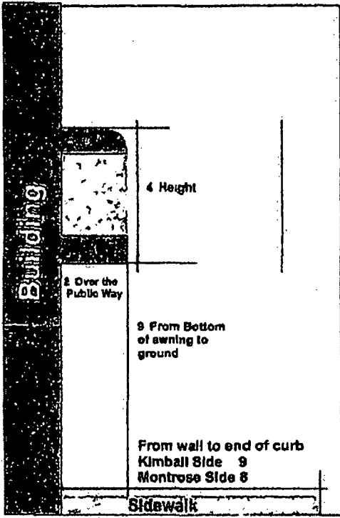
1 Standard Awning constructed of galvanized steel frame 1" square tube Translucent Awning Vinyl sewn and wrapped on awning frame
