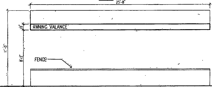
FRONT ELEVATION
