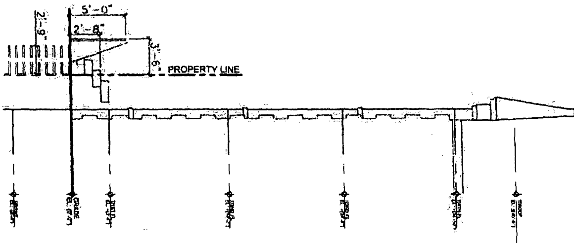
Front Buildings WEST ELEVATION
