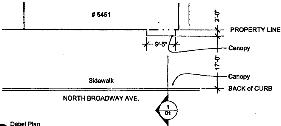
Detail Plan Scale 1/16" = 1'
