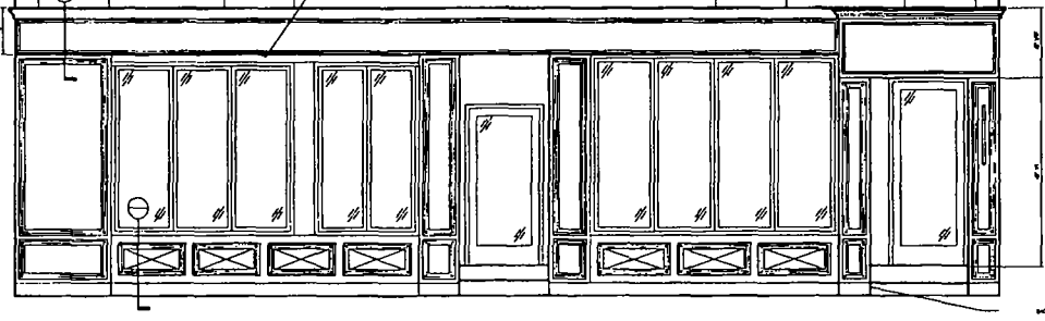
F2 FRONT ELEVATION
