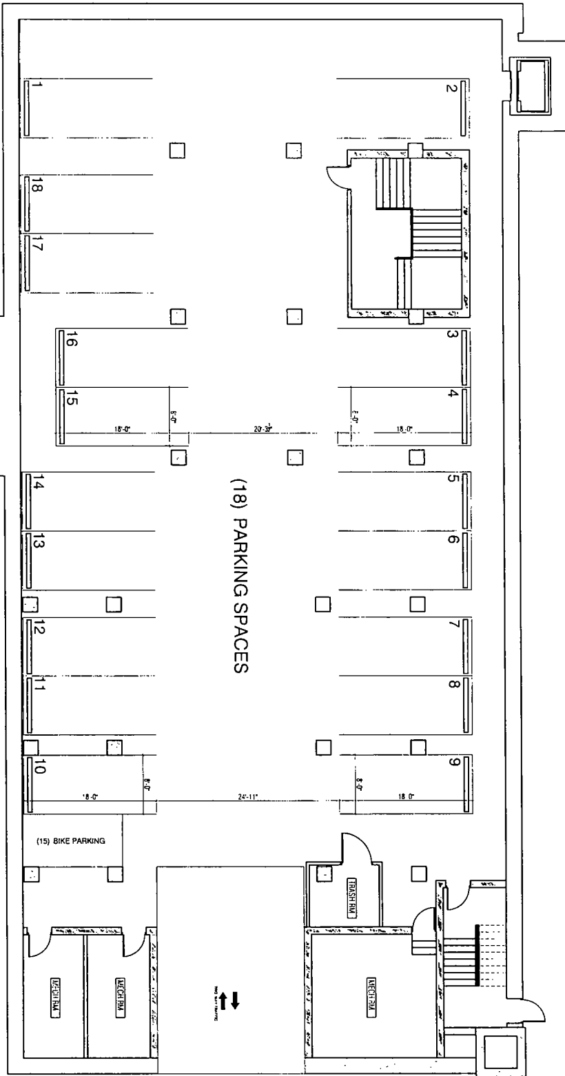
BASEMENT FLOOR PLAN 1/4" = 1'-0"
