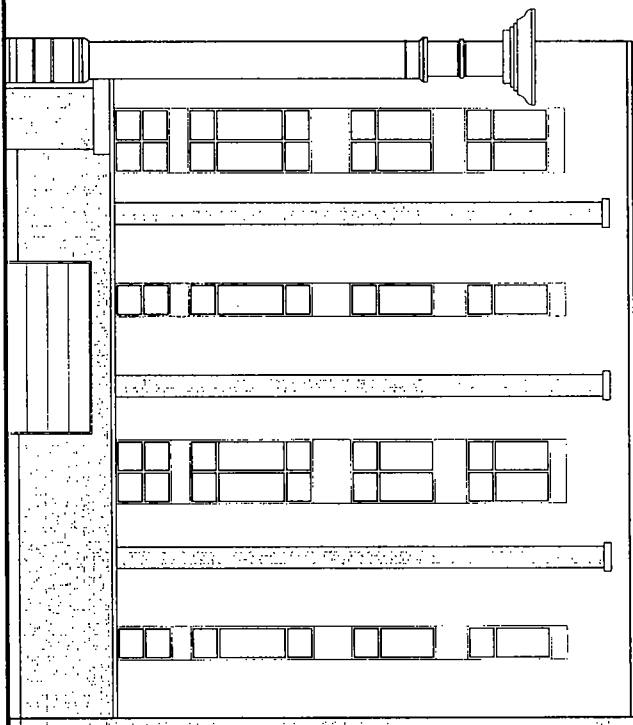
EAST ELEVATION 1/4" = 1'-0"
