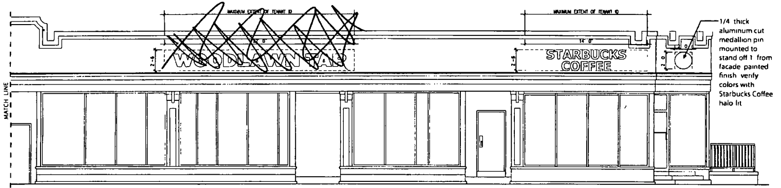
SOUTH (FRONT) ELEVATION 3/16" = 1' 0"
