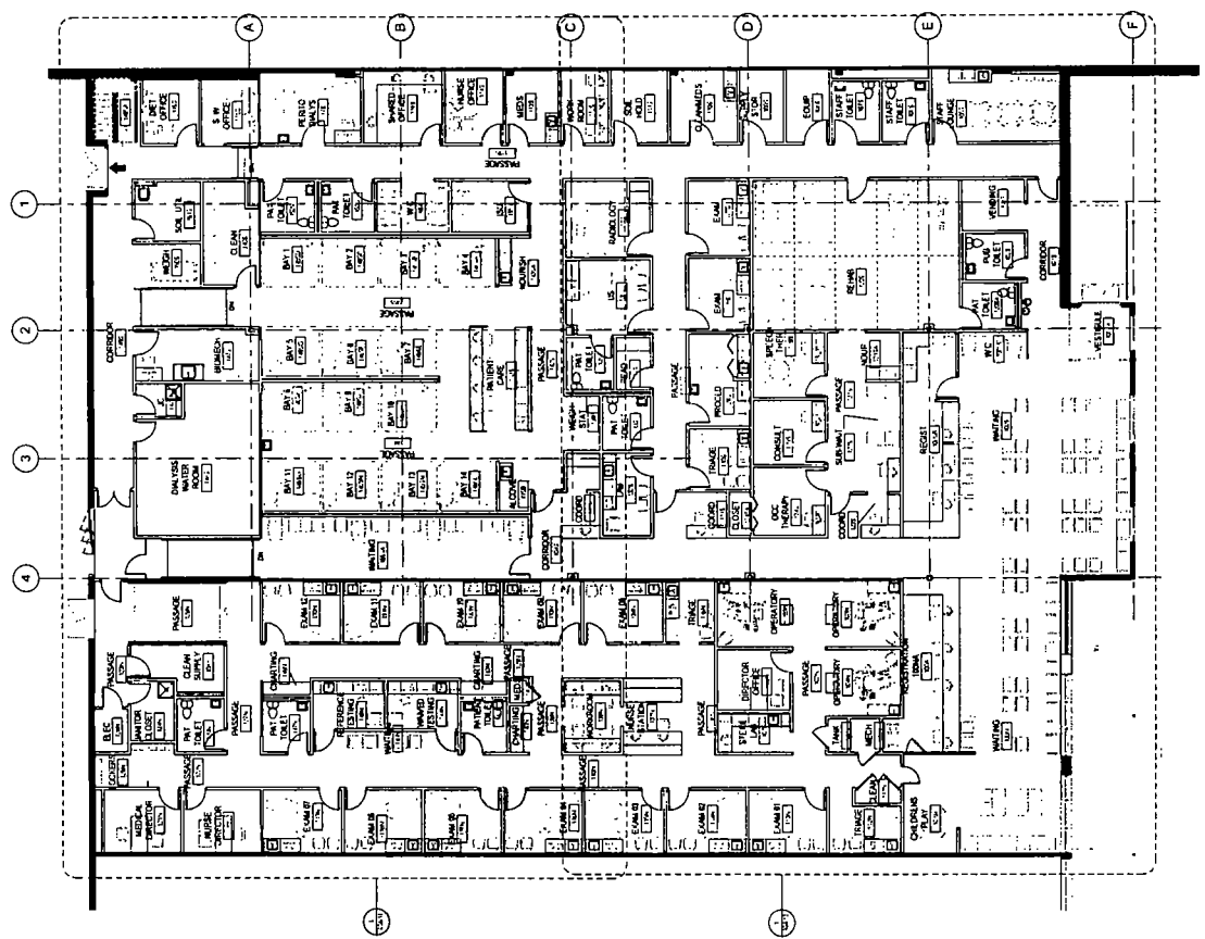
① LEVEL 01 - FLOOR PLAN REV. 11.07
