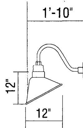
LIGHT FIXTURE DETAIL 3/4" = 1'-0"
