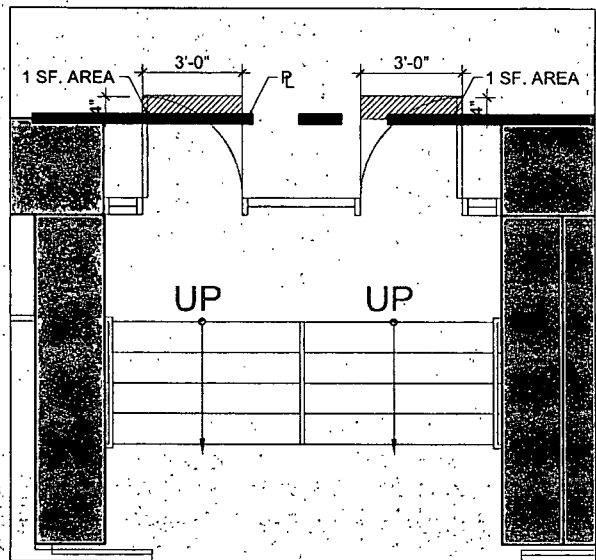
NEW STOREFRONT REPLACEMENT DOORS ALONG OHIO STREET
