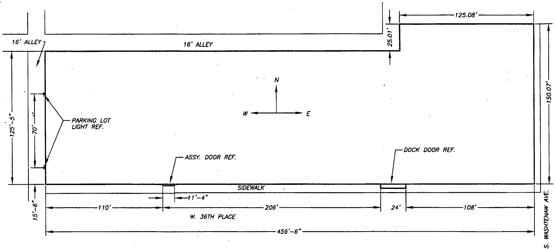
PLAN VIEW
