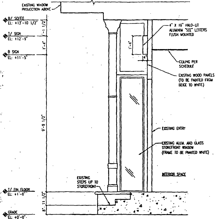
FB SECTION @ MAIN ENTRY SCALE: 3/8" = 1'-0"
