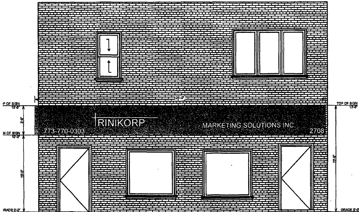
NORTH ELEVATION 1 NOT TO SCALE (A-1)
