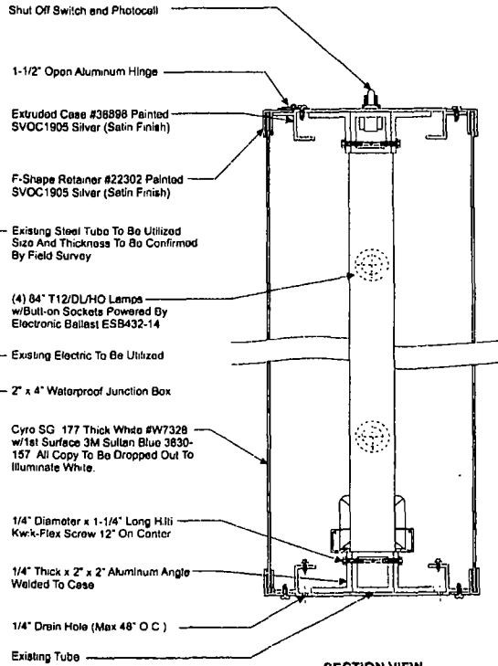
SECTION VIEW SCALE 3\"/>
