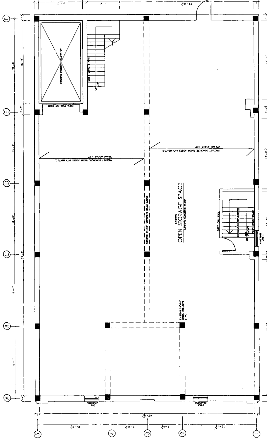
EXISTING 5th FLOOR PLAN SCALE: 1/8"=1'-0"
