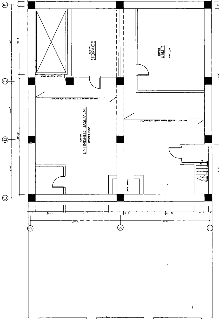
EXISTING BASEMENT PLAN SCALE: 1/8"=1'-0"
