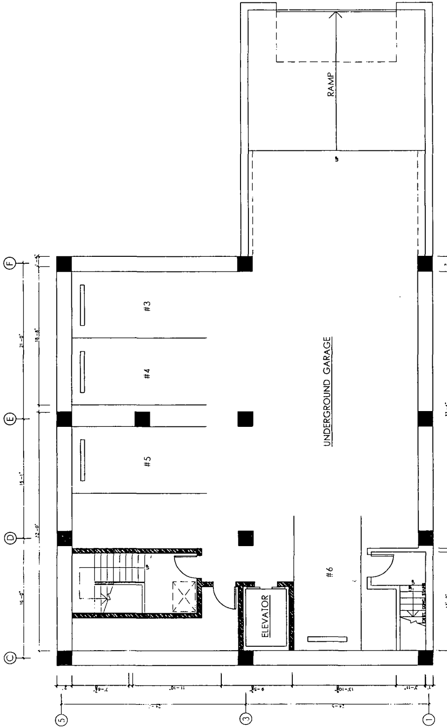
BASEMENT FLOOR PLAN SCALE: 1/8"=1'-0"
