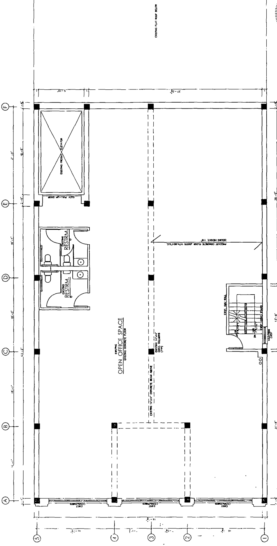
EXISTING 2nd FLOOR PLAN SCALE: 1/8" = 1'-0"
