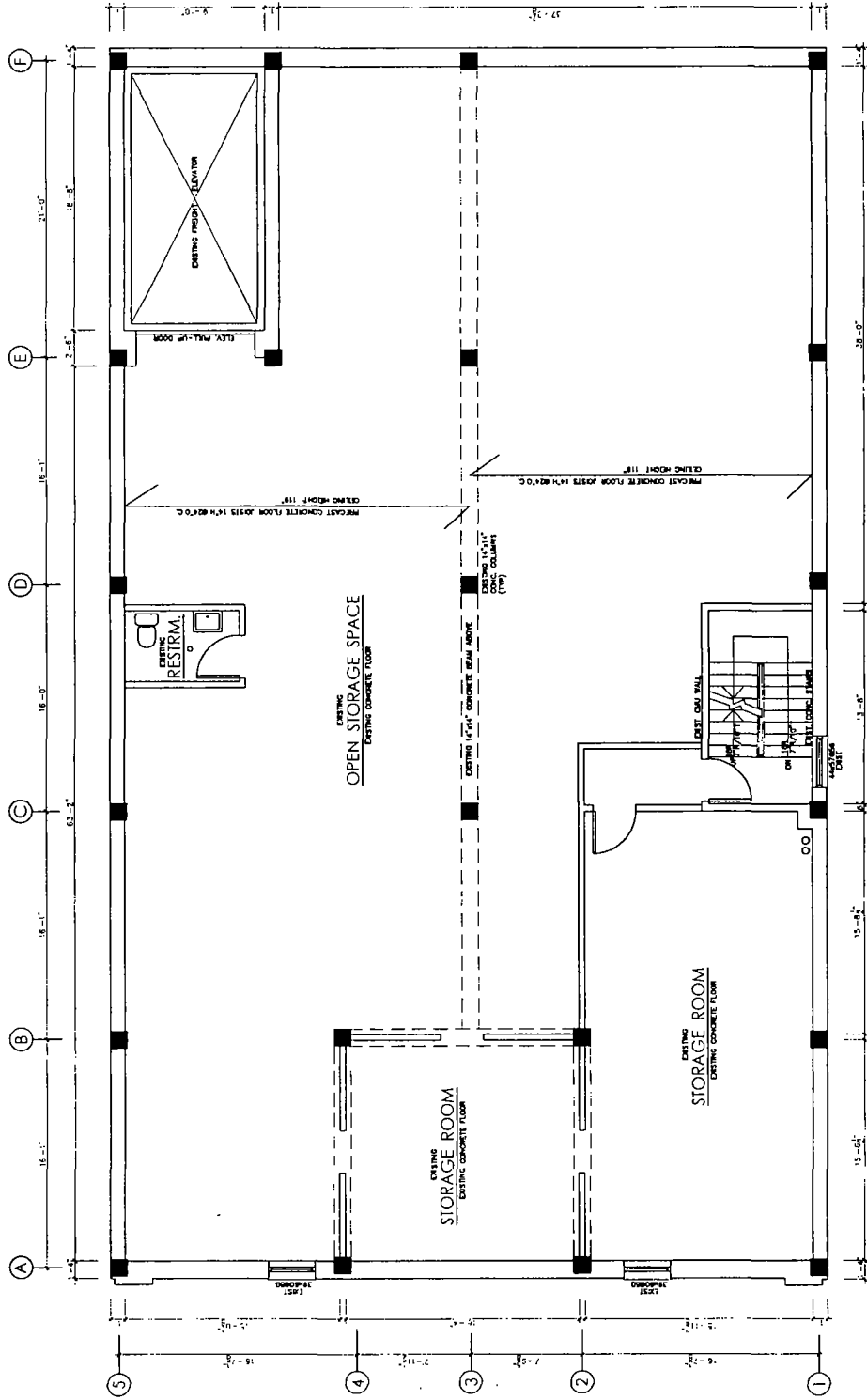
EXISTING 4th FLOOR PLAN SCALE 1/8"=1'-0"
