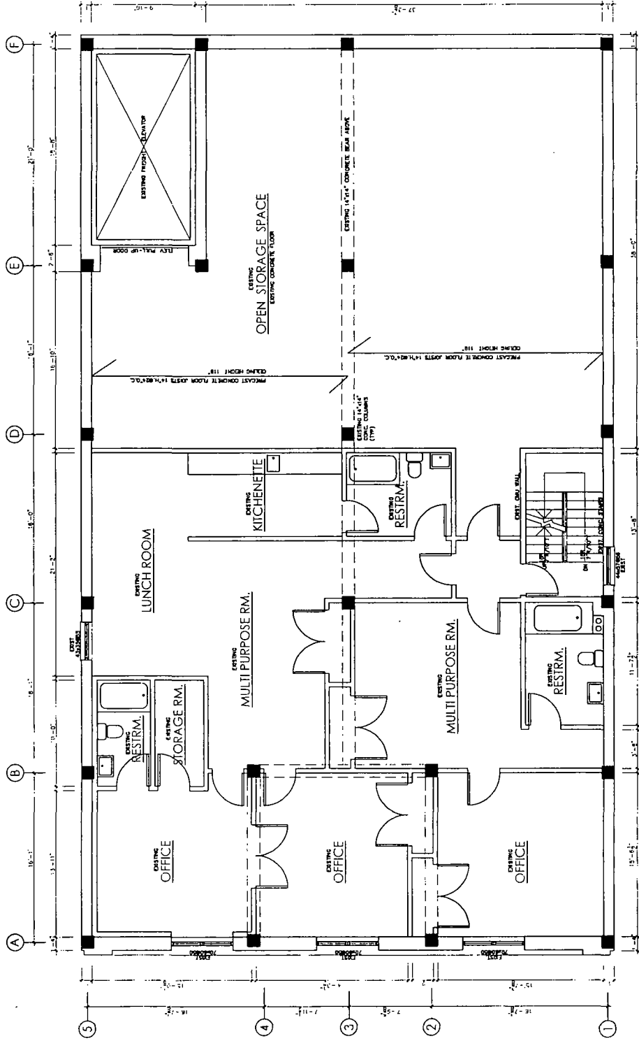
EXISTING 3rd FLOOR PLAN SCALE: 1/8"=1'-0"
