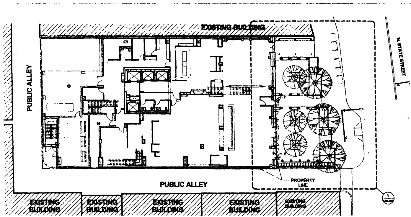
1 SITE PLAN 1/16" = 1'-0"
