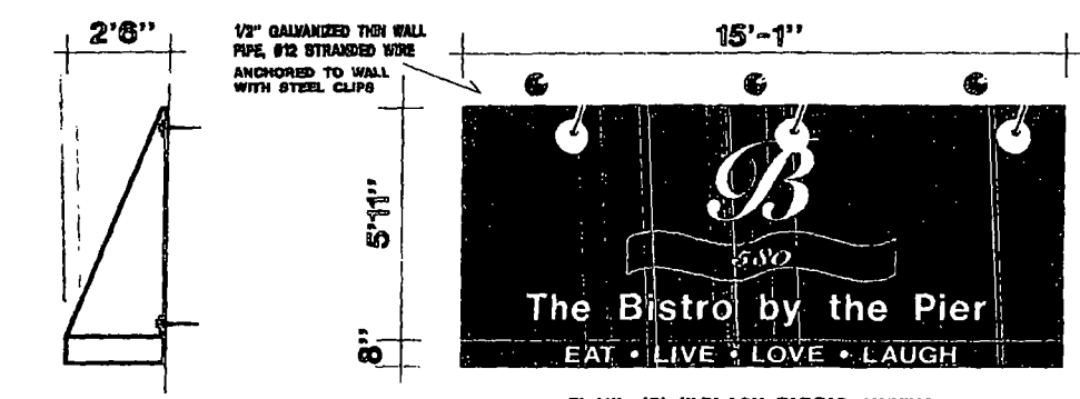
SIDE VIEW SHOWING CLIPS AND 3/8" EXPANSION BOLTS USED TO MOUNT AWNING
