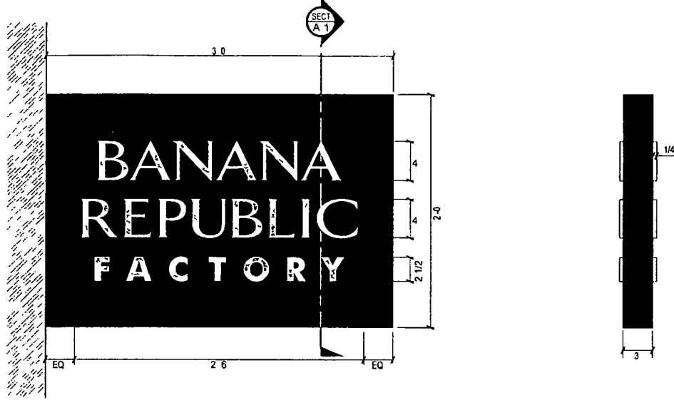
C TYPE C CUSTOM FABRICATED D/F ALUM BLADE SIGN w/ PUSH THRU ILLUM LOGO - FLAG MOUNT - TYP SIDE & END ELEVATIONS Scale 1 1/2" = 1'-0"
