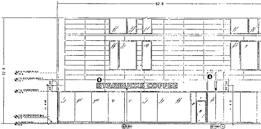
4 WEST ELEVATION Scale 1/8" = 1"
