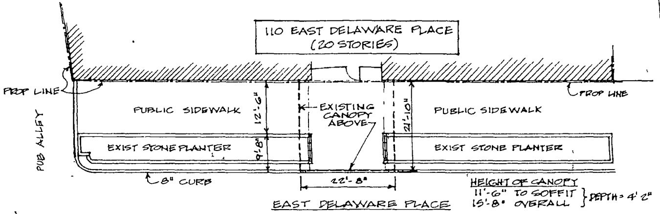
PLAN OF PUBLIC WAY SCALE: 1/16" = 1'-0"
