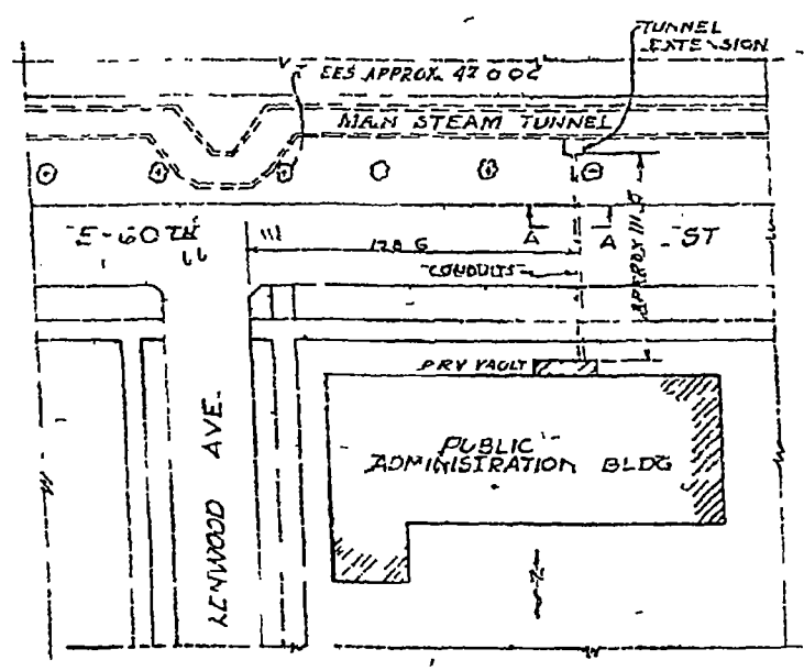
PART PLOT PLAN SCALE 1/500'
