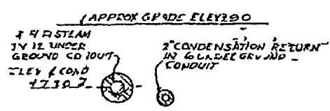
SECTION "A-A" SCALE 3/16"
