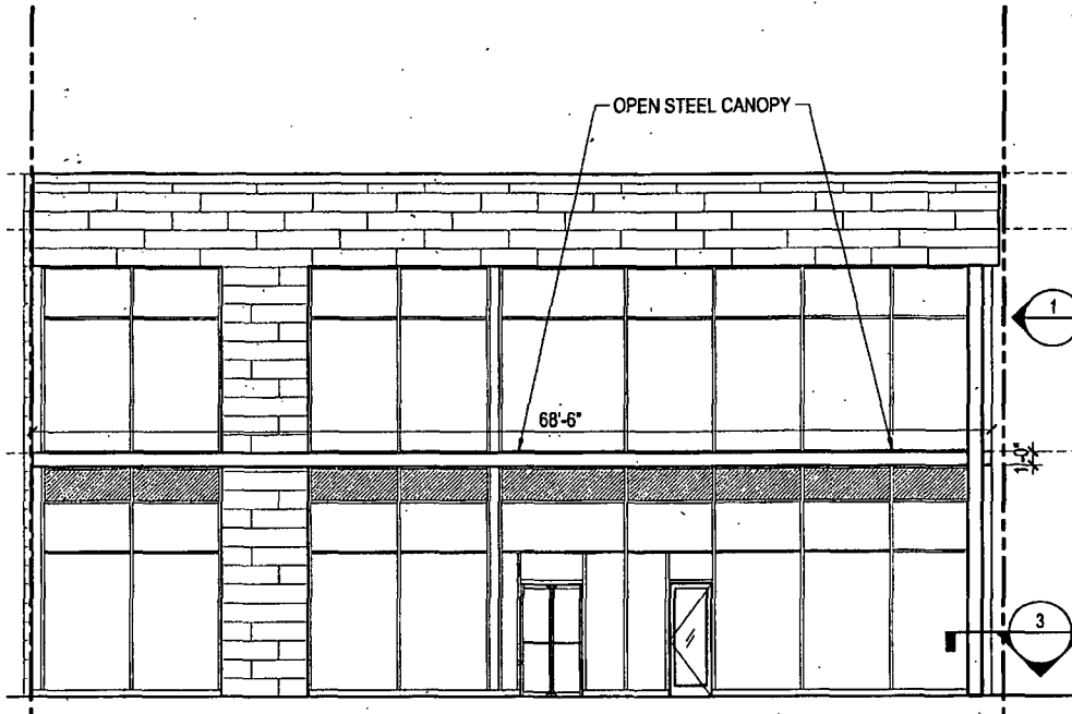
2 North Elevation SCALE 3/32"=1'-0"
