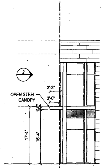
1 Partial West Elevation SCALE 3/32"=1'-0"
