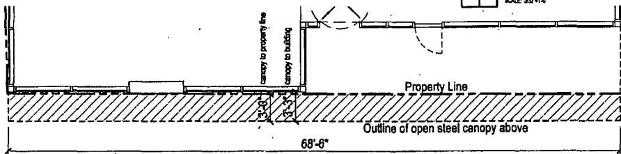
3 Plan at North Elevation SCALE 3/32"=1'-0"
