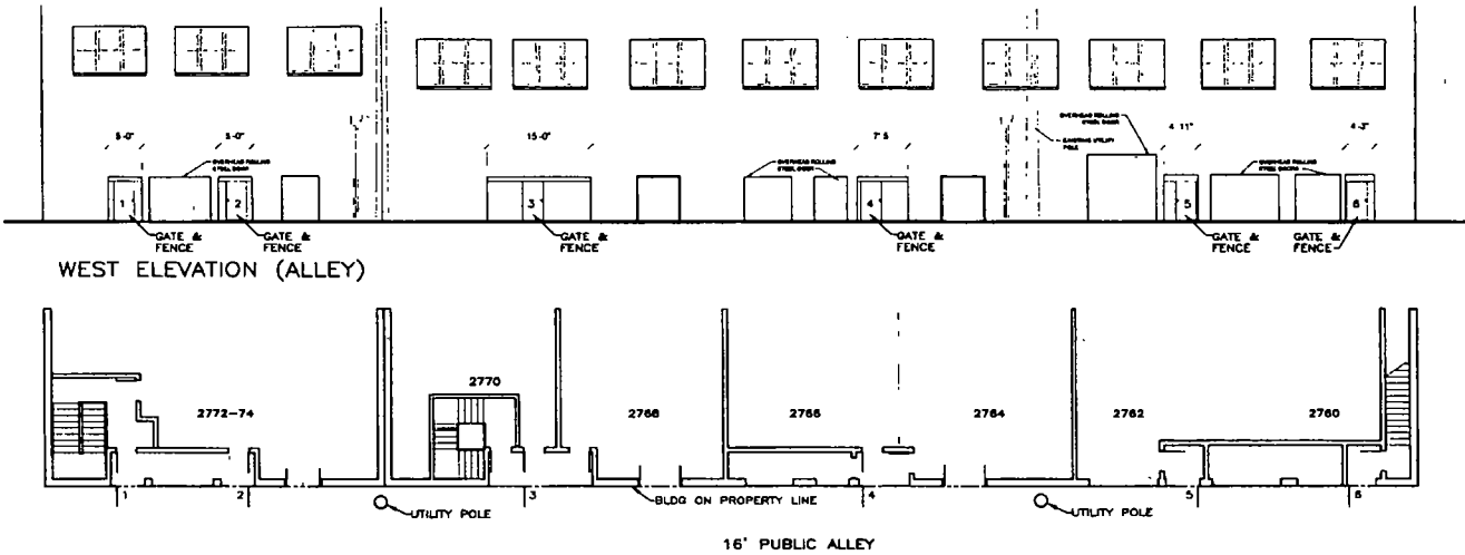
PLAN OF BACK OF 2760-74 N MILWAUKEE (AT ALLEY)
