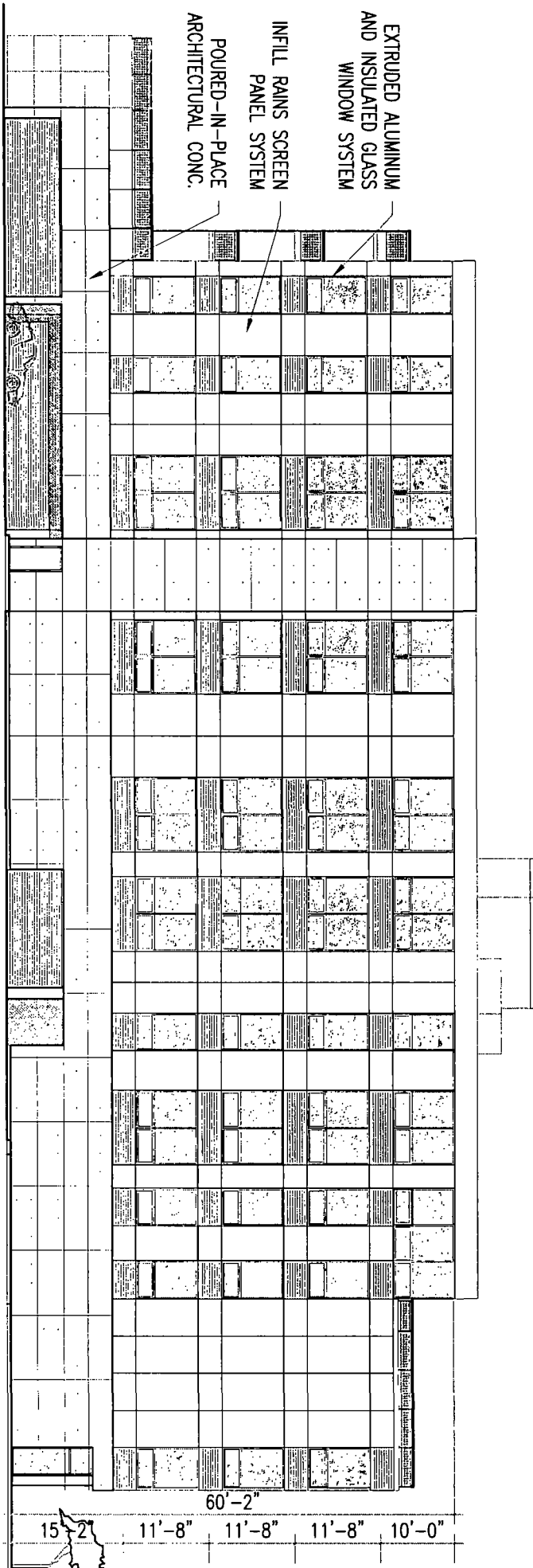
ALLEY ELEVATION
