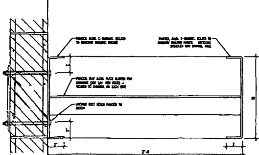
INSTALLATION DETAIL INSTALLED WITH 1/2"x5" THROUGH BOLTS AS SHOWN
