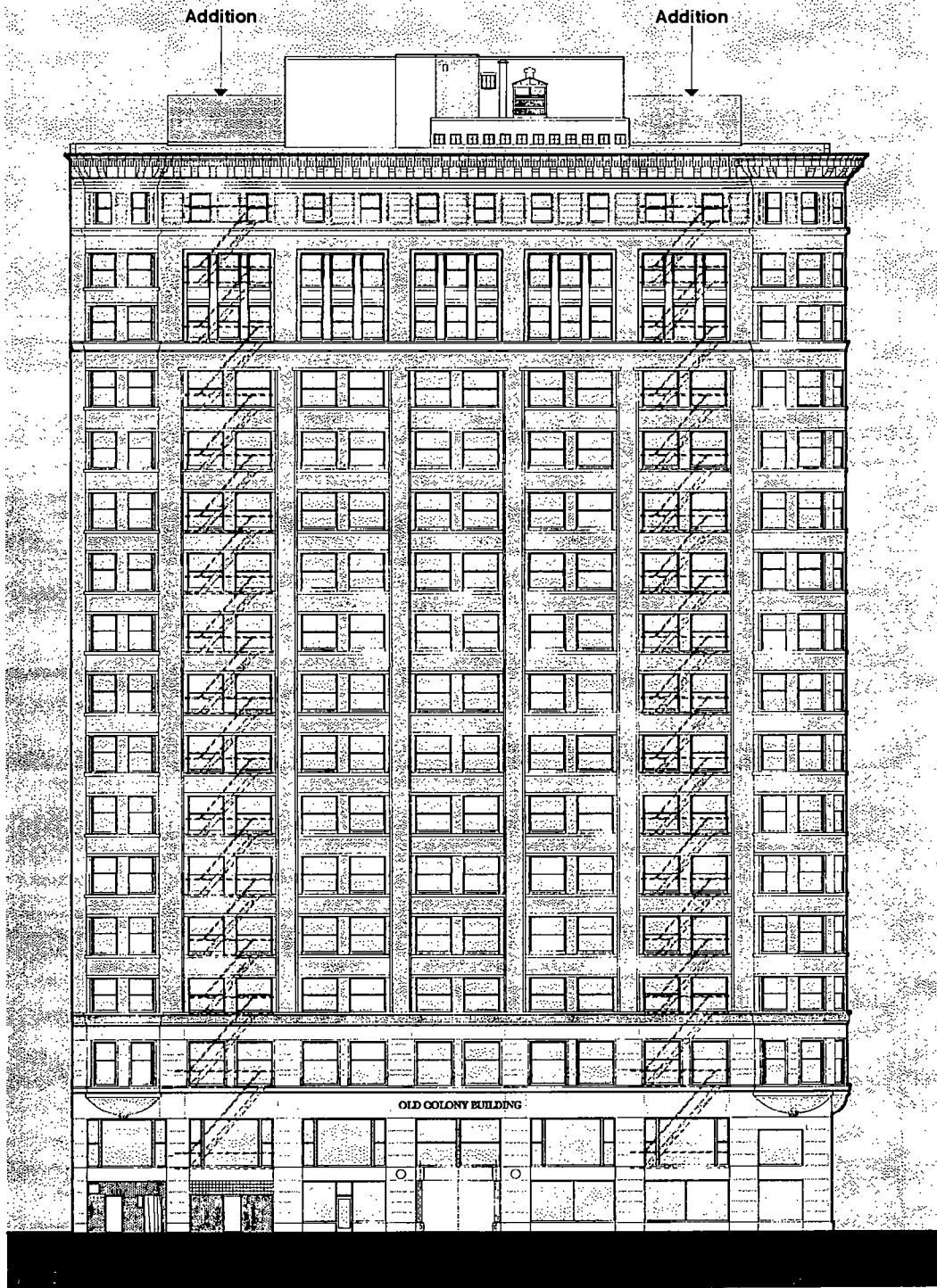
East (Plymouth) Elevation
