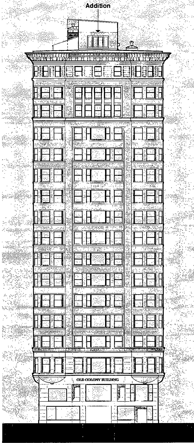
North (Van Buren) Elevation 1" = 30'
