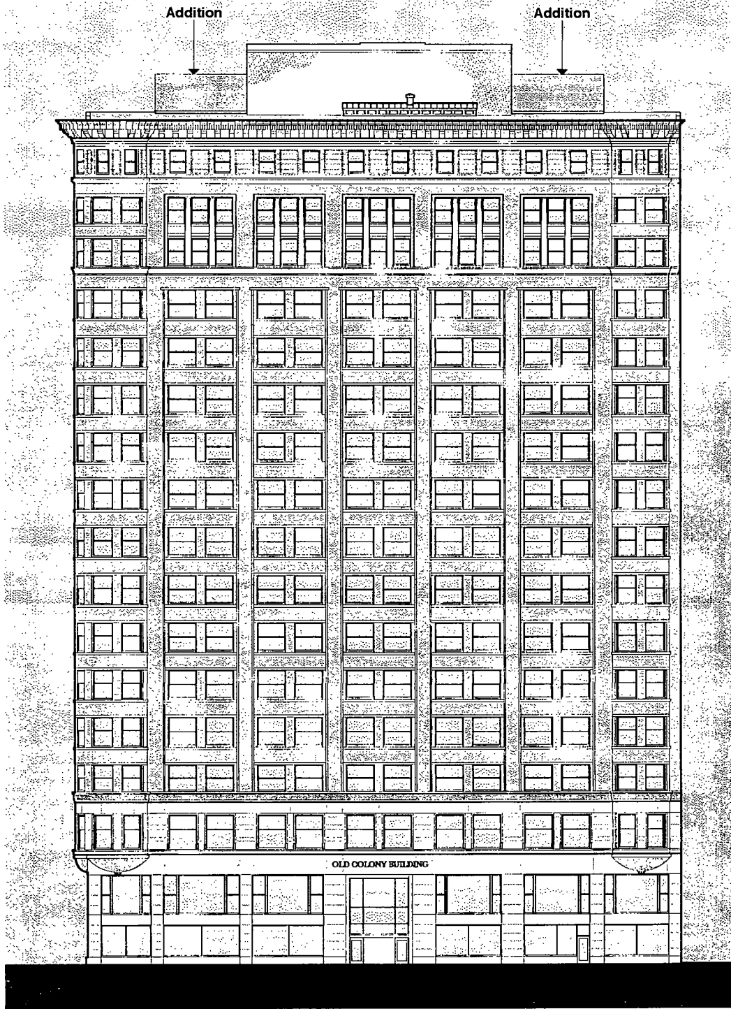
West (Dearborn) Elevation
