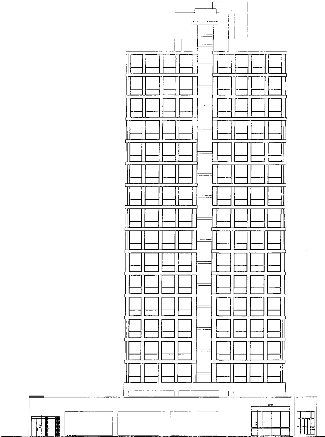
WEST ELEVATION
