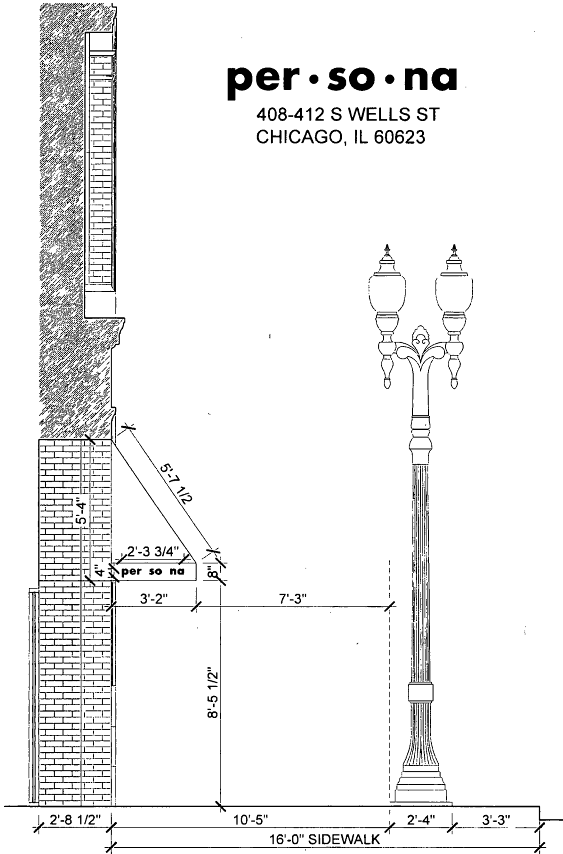
2 SIDE ELEVATION NTS
