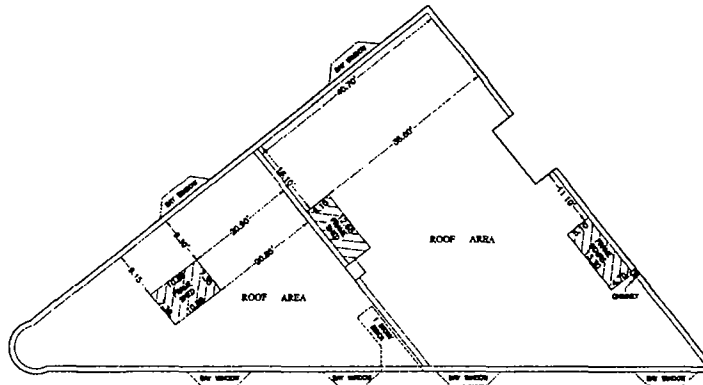
DETAIL ON ROOF LEVEL
