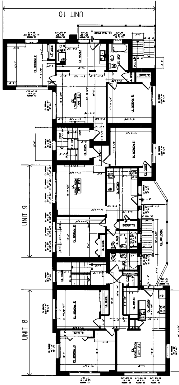
EXISTING THIRD FLOOR PLAN WITH (3) EXISTING DWELLING UNITS 3/18/10
