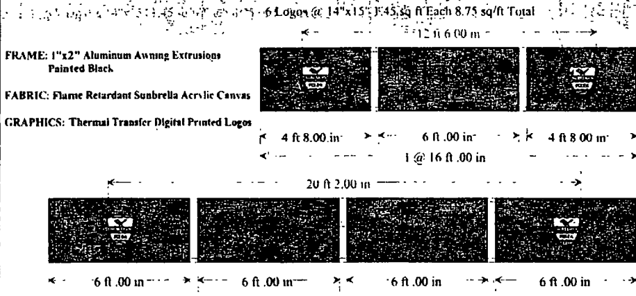
Continuous Awning Frame with Separation Between Fabric Sections
