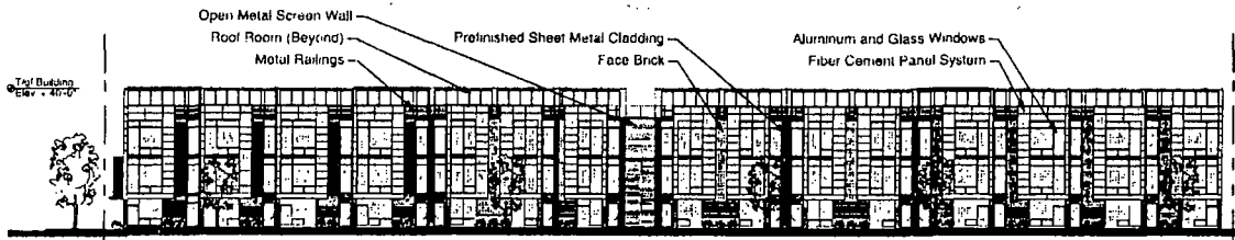
North Elevation - North Car Court
