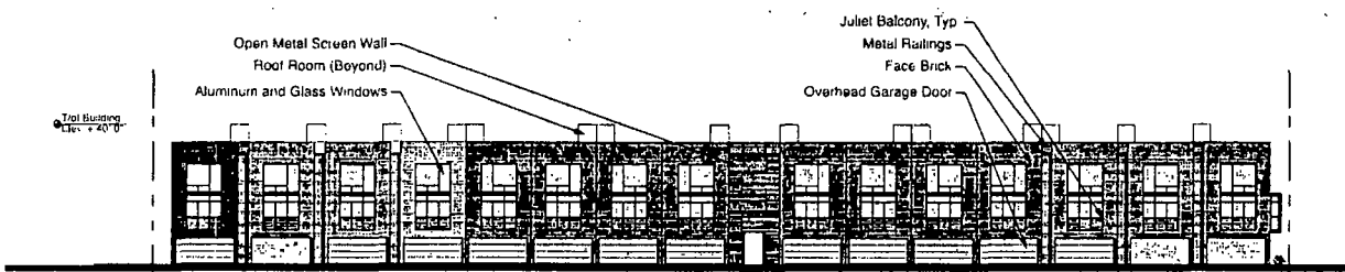
North Elevation - North Car Court
