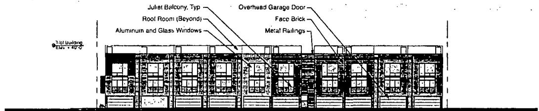
South Elevation - South Car Court South Elevation - Public Alley
