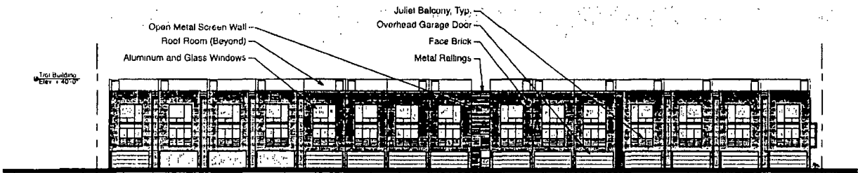
North Elevation - Public Alley
