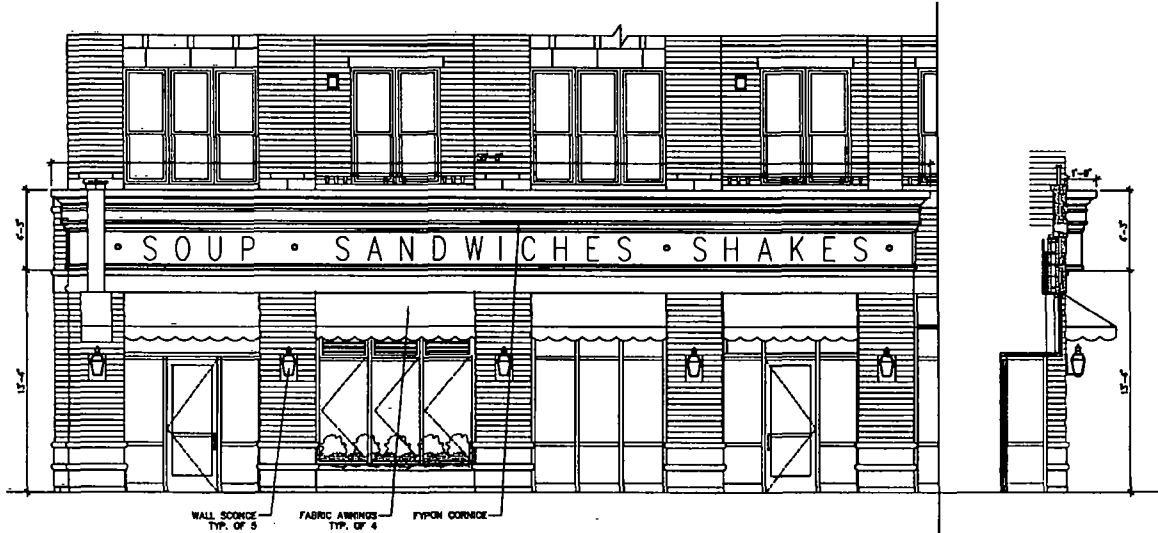
EXTERIOR ELEVATION
