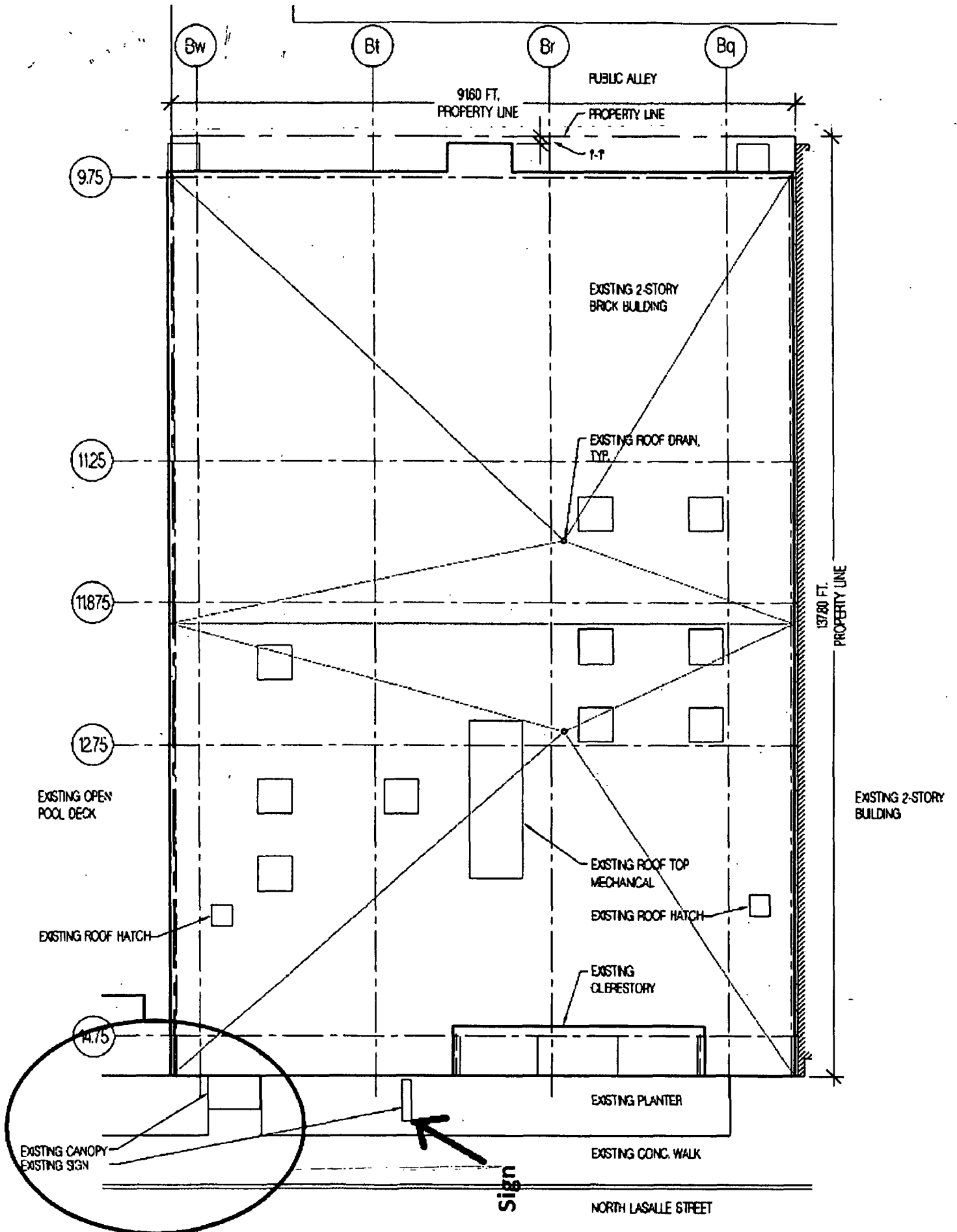
1 | SITE PLAN
