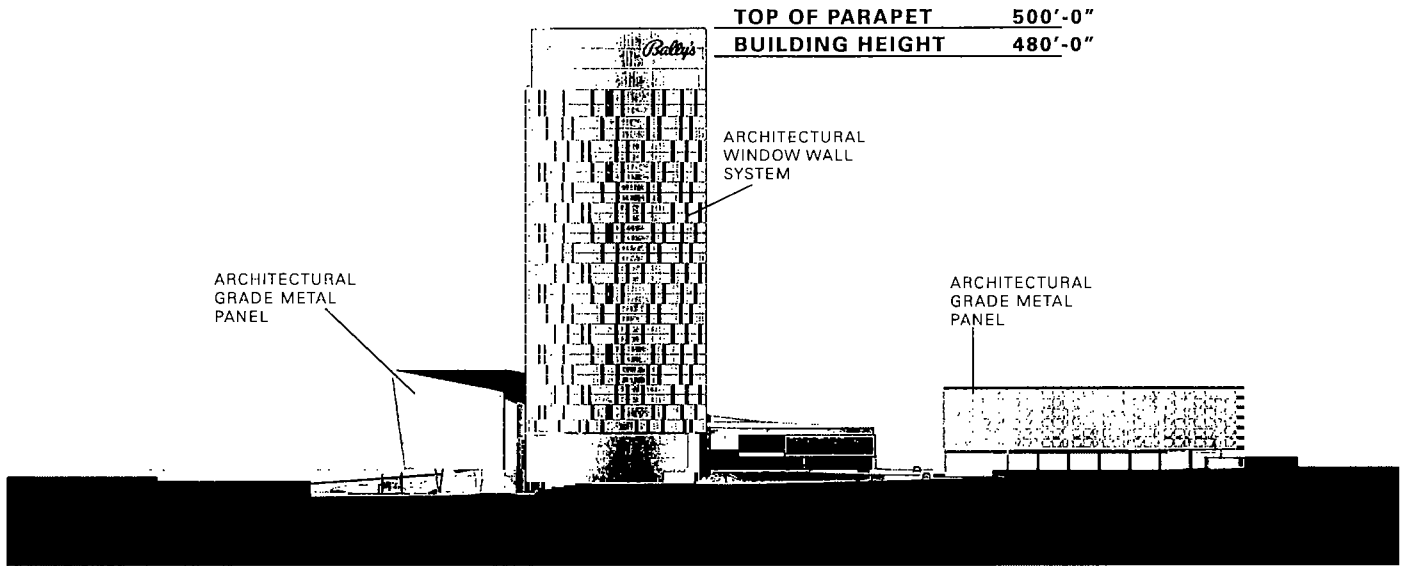
NORTH ELEVATION
