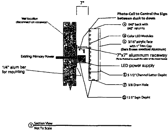
Typical Raceway Mount channel Letters with LED's
